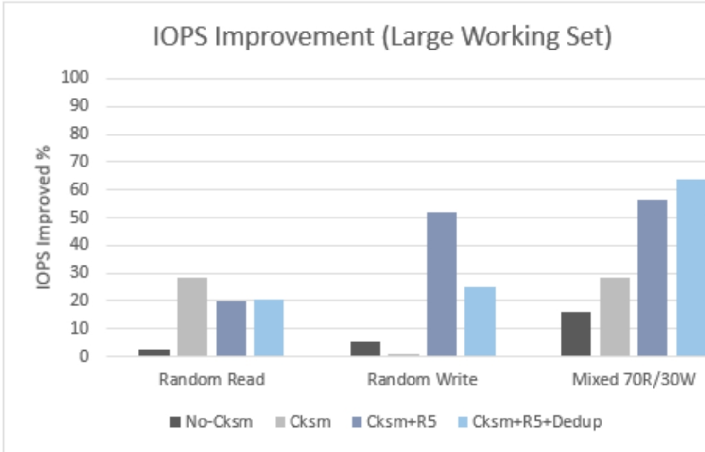
Figure 1. Improvement (%) in IOPS for vSAN 6.6 over vSAN 6.5 – Large working sets Moved Permanently The document has moved here .
